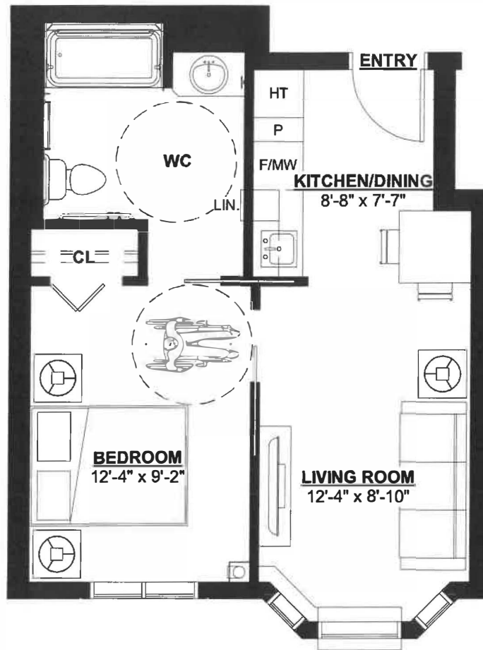
SUITE G ONE BEDROOM SUITE SUITE AREA 454 S.F. Units 208, 308, 408, 508
