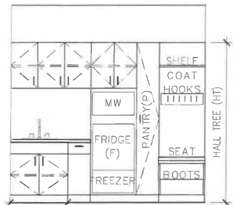
REMOVABLE CABINET
