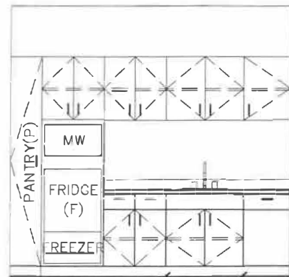
KITCHEN ELEVATION
